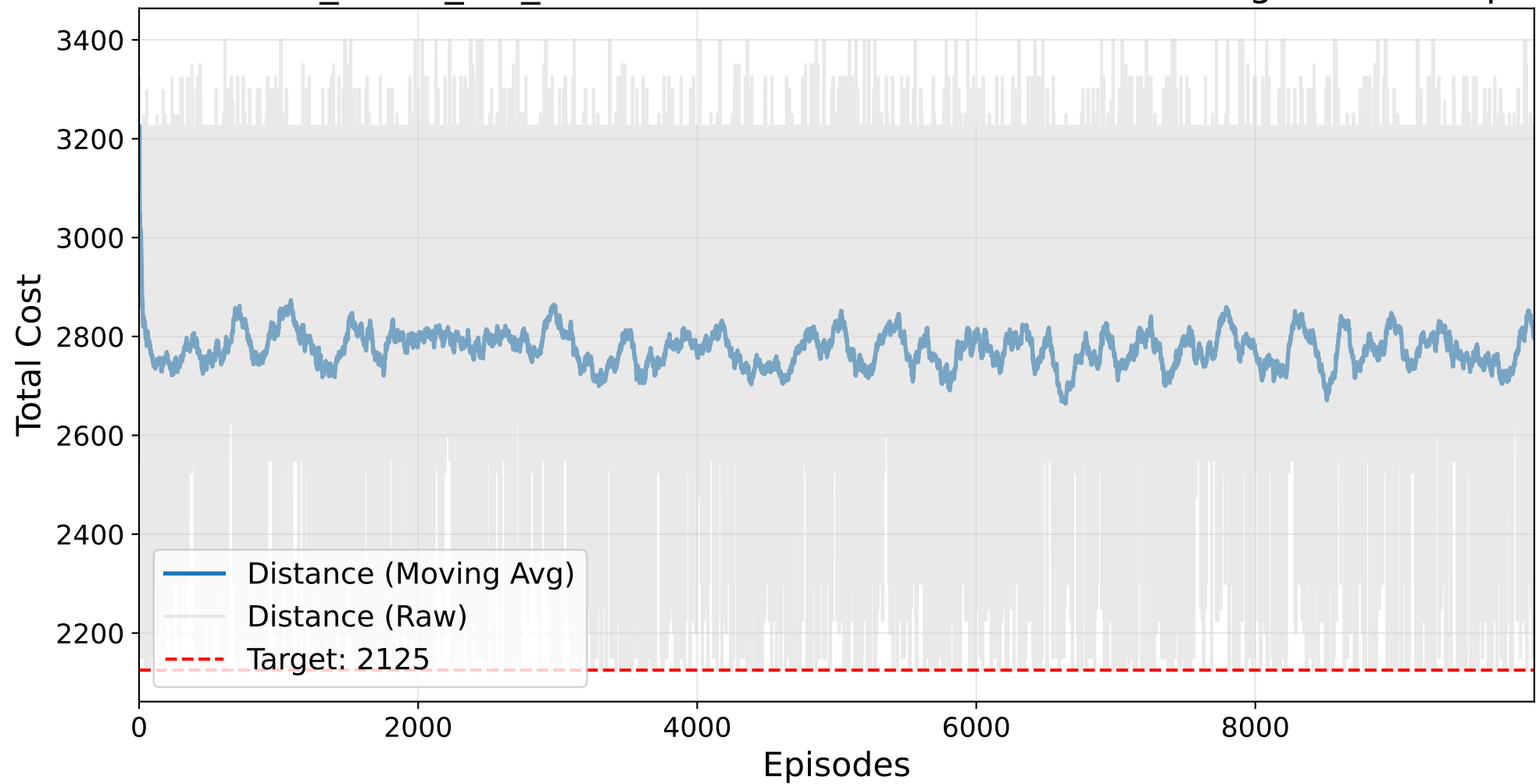
Final NO_MASK_NO_BAYESIAN Masked AutoRL-SOP Training - ESC07.sop
